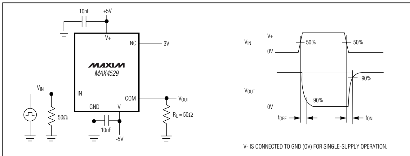
Figure 2. Switching Time
