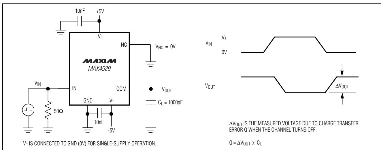
Figure 3. Charge Injection
